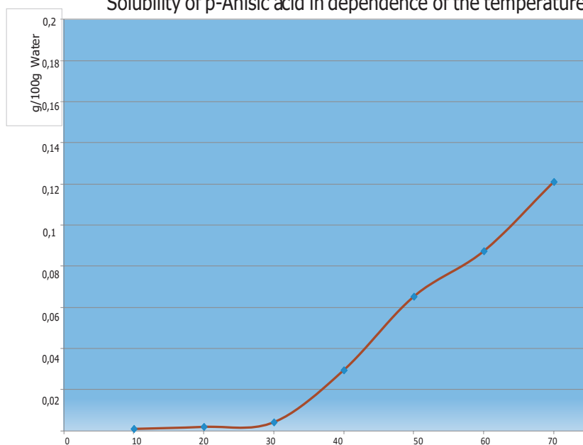
Solubility of p-Anisic acid in dependence of the temperature
